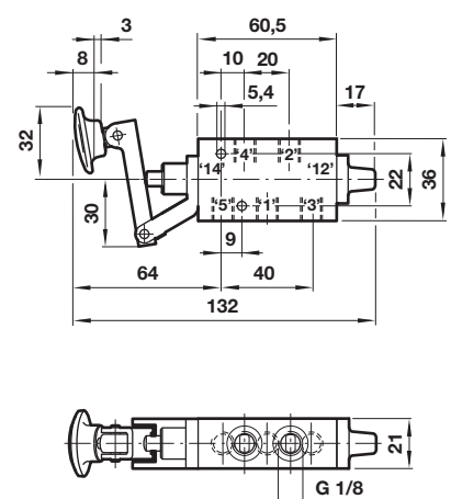
X3046602 5/2 Lever operated spring return valve
