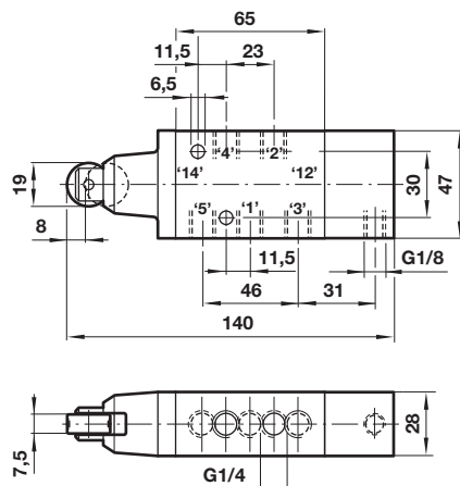
X3064902 5/2 Roller actuated pilot return valve
